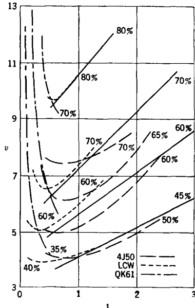
FIG. 10-40.—Collected efficiency contours for N = 16 . \sigma = 0.60 to 0.66 .
